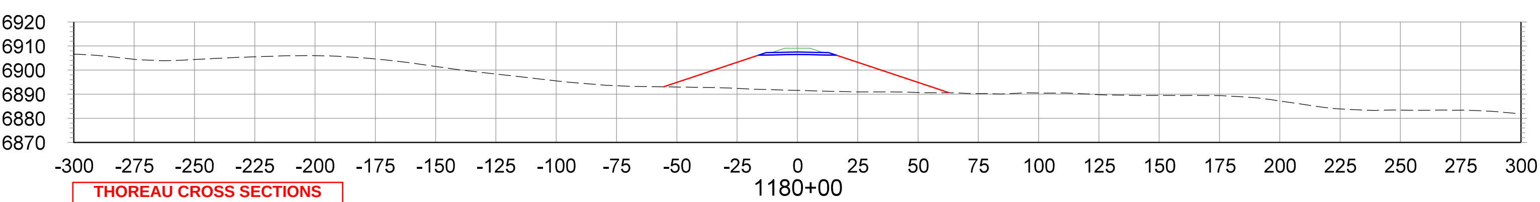
CROSS SECTIONS STA.1180+00 TO STA.1195+00
