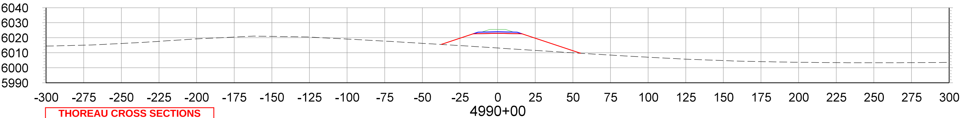
CROSS SECTIONS STA.4990+00 TO STA.5005+00
