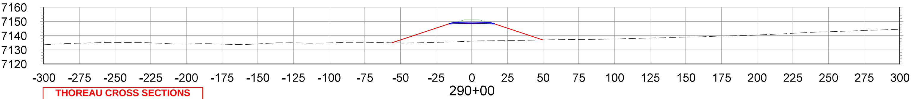
CROSS SECTIONS STA.290+00 TO STA.305+00
