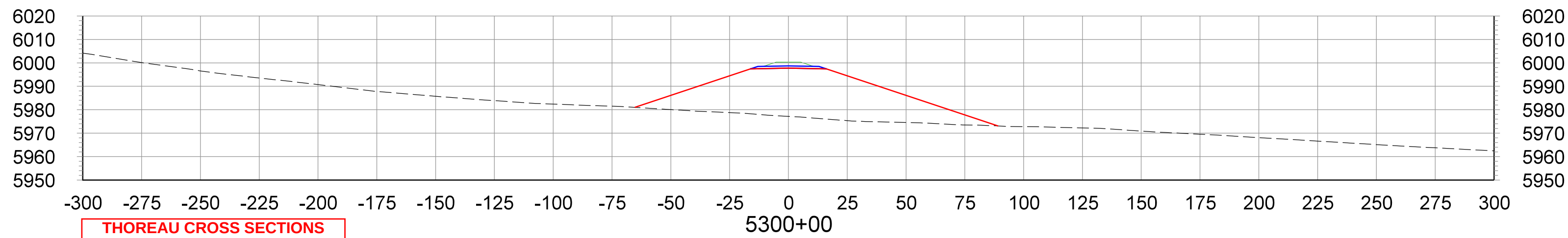
CROSS SECTIONS STA.5300+00 TO STA.5310+00
