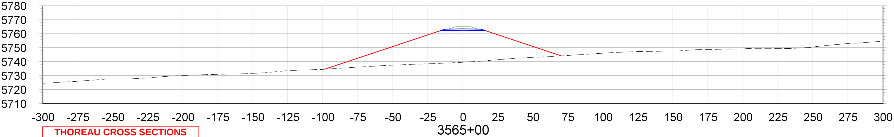
CROSS SECTIONS STA.3565+00 TO STA.3580+00
