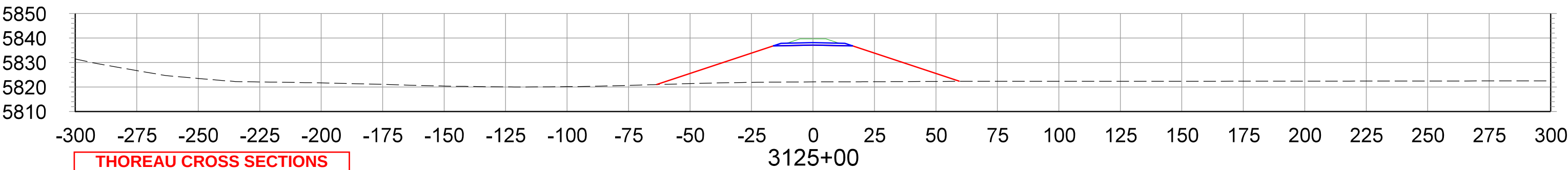
CROSS SECTIONS STA.3125+00 TO STA.3140+00
