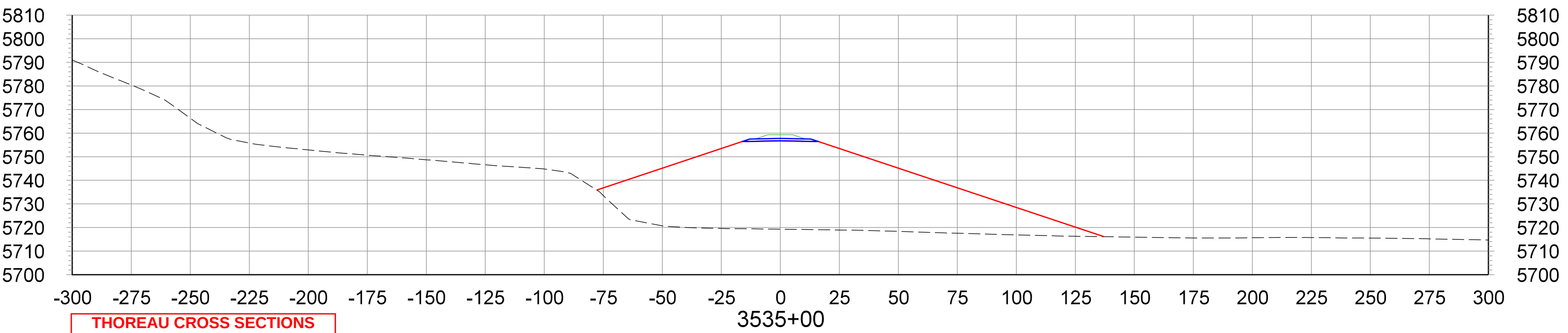
CROSS SECTIONS STA.3535+00 TO STA.3545+00
