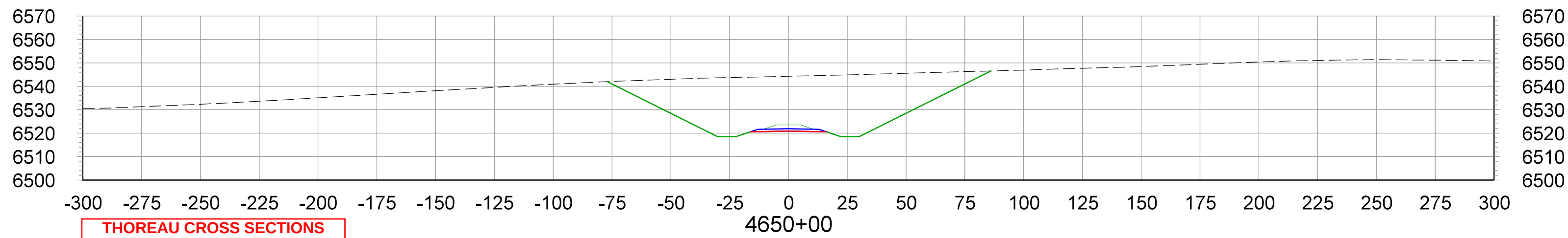
CROSS SECTIONS STA.4650+00 TO STA.4660+00
