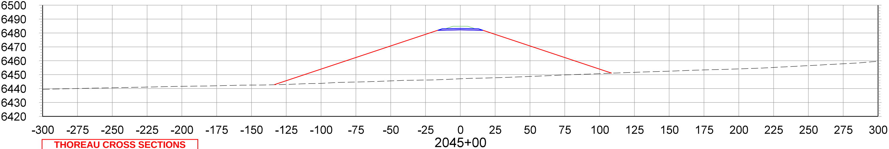
CROSS SECTIONS STA.2045+00 TO STA.2060+00
