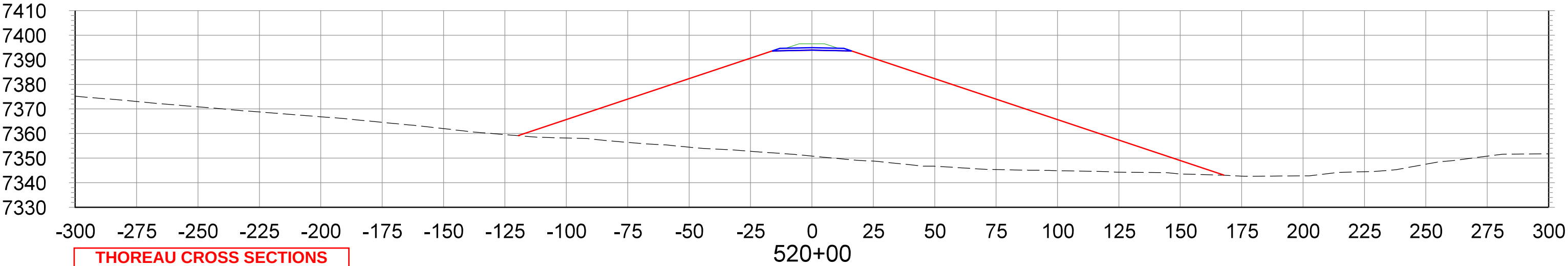
CROSS SECTIONS STA.520+00 TO STA.535+00
