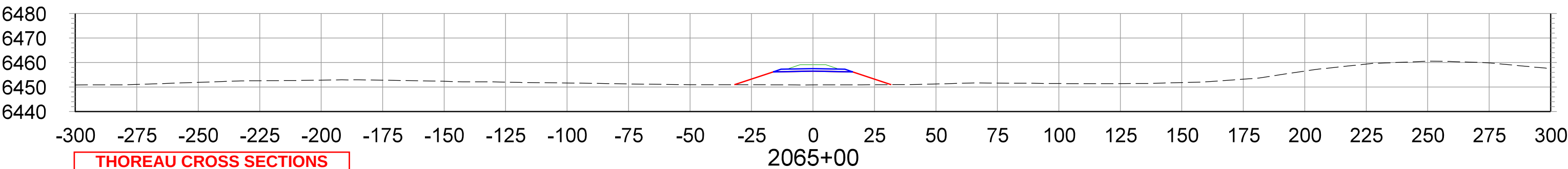
CROSS SECTIONS STA.2065+00 TO STA.2080+00
