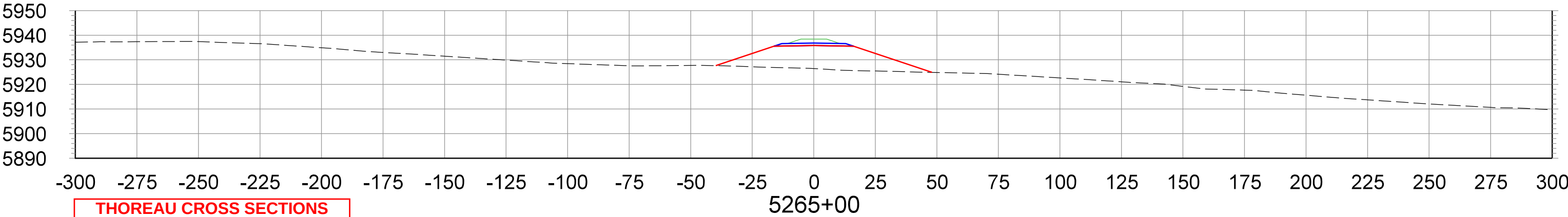
CROSS SECTIONS STA.5265+00 TO STA.5280+00
