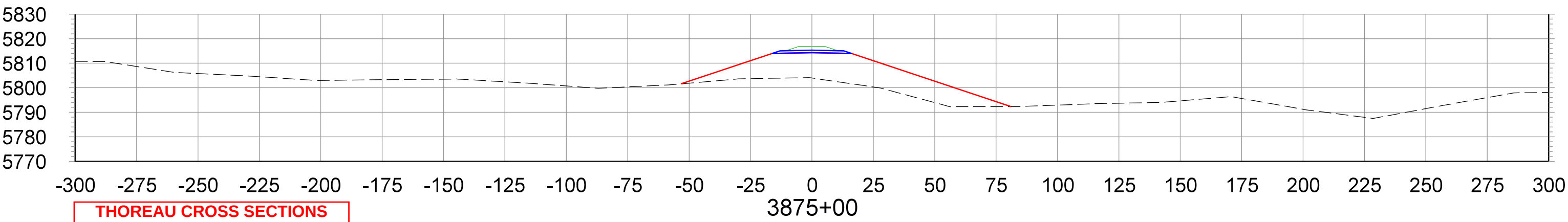
CROSS SECTIONS STA.3875+00 TO STA.3890+00
