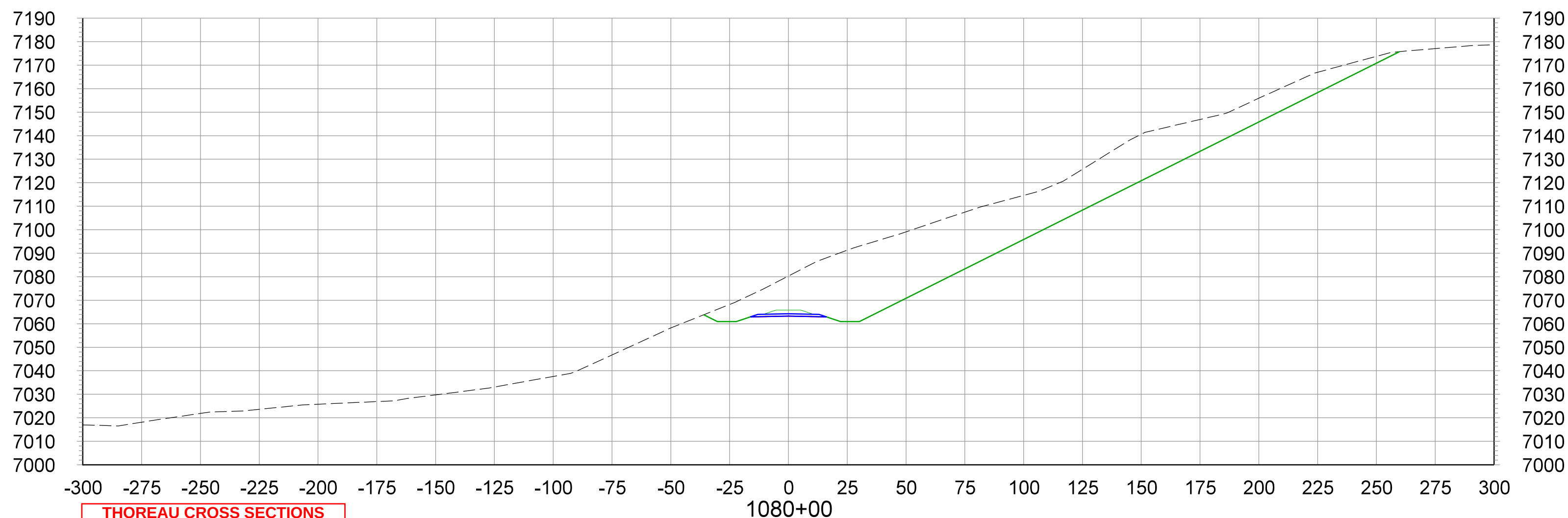
CROSS SECTIONS STA.1080+00 TO STA.1085+00
