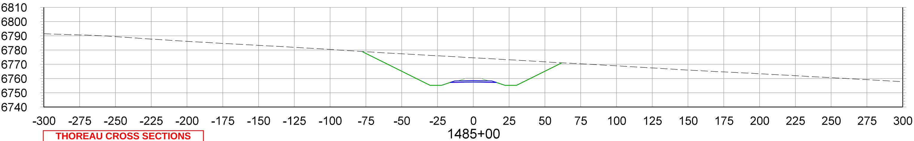
CROSS SECTIONS STA.1485+00 TO STA.1500+00
