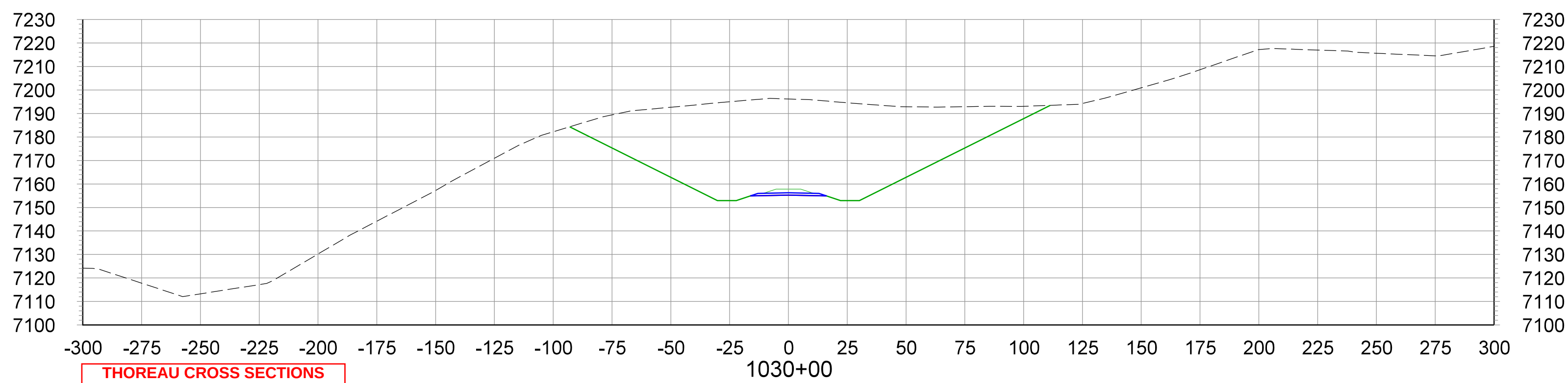
CROSS SECTIONS STA.1030+00 TO STA.1035+00
