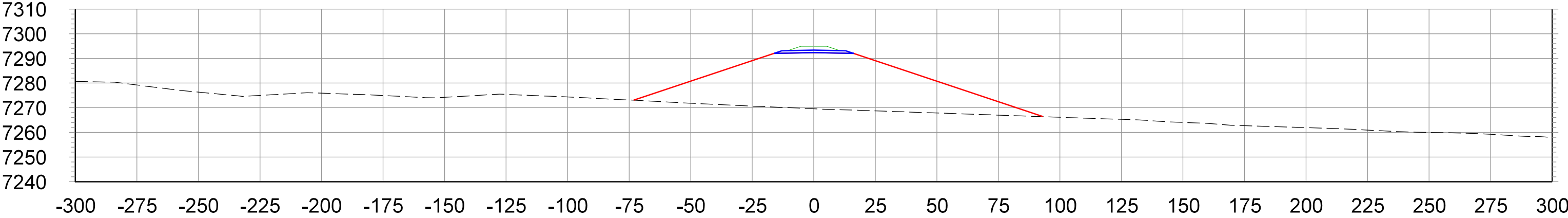
CROSS SECTIONS STA.595+00 TO STA.610+00
